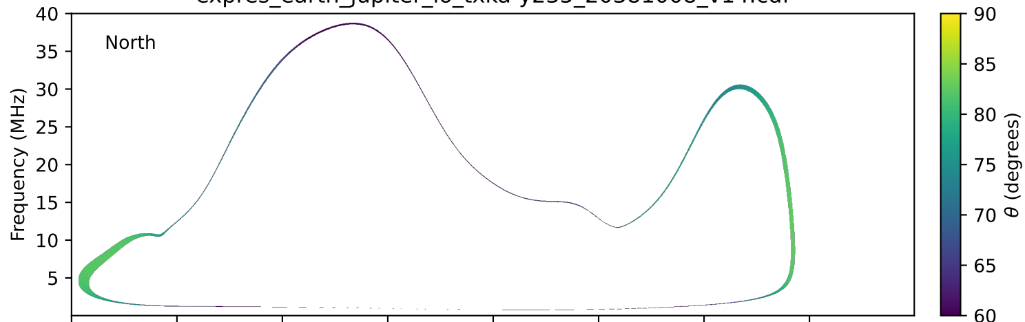
expres_earth_jupiter_io_txka-y235_20381008_v14.cdf
