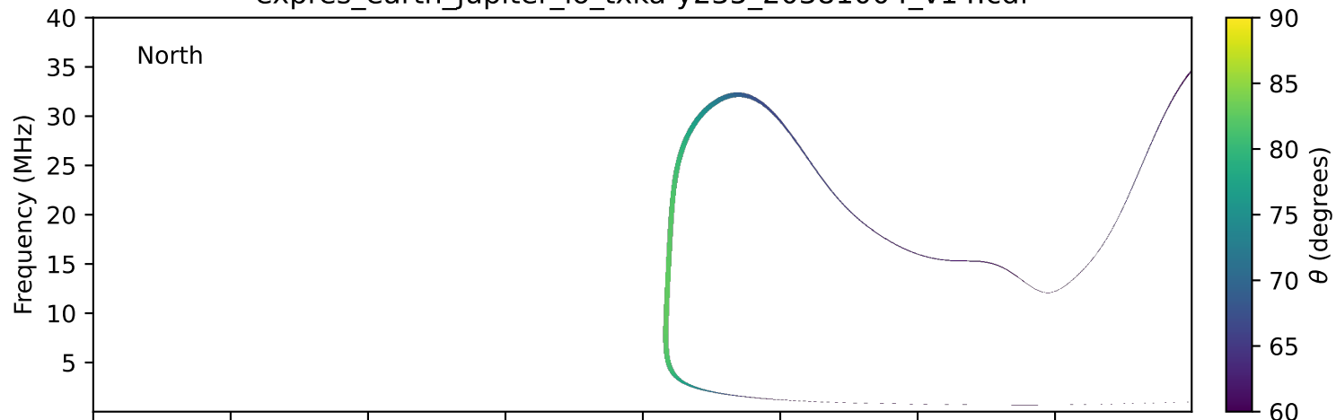
expres_earth_jupiter_io_txka-y235_20381004_v14.cdf
