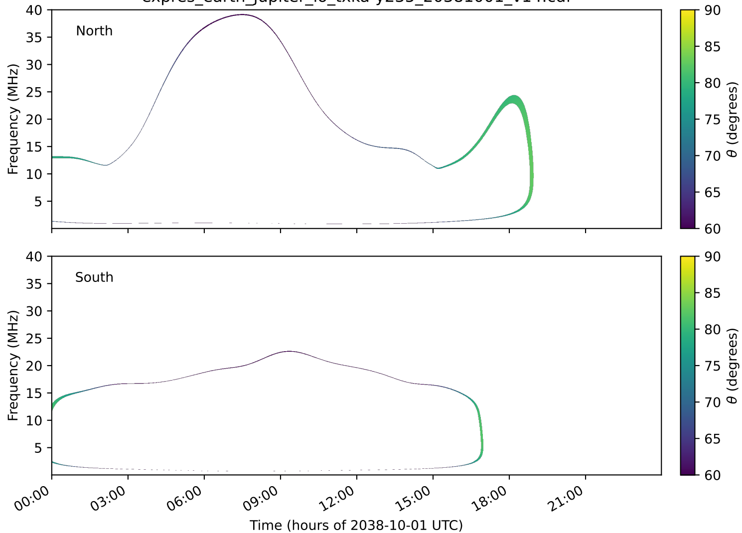
expres_earth_jupiter_io_txka-y235_20381001_v14.cdf
