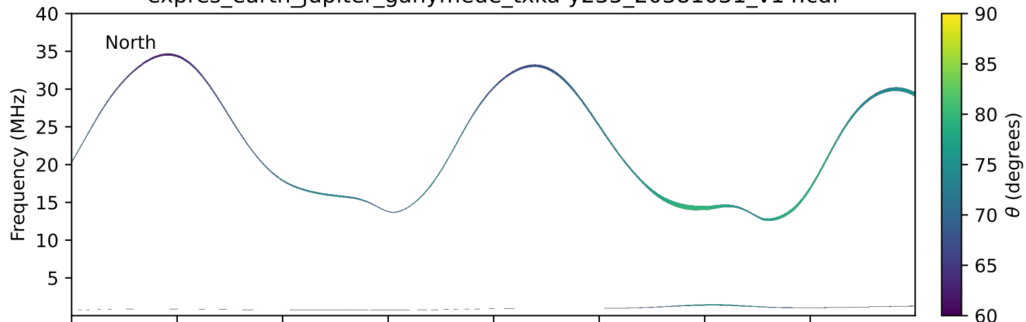
expres_earth_jupiter_ganymede_txka-y235_20381031_v14.cdf
