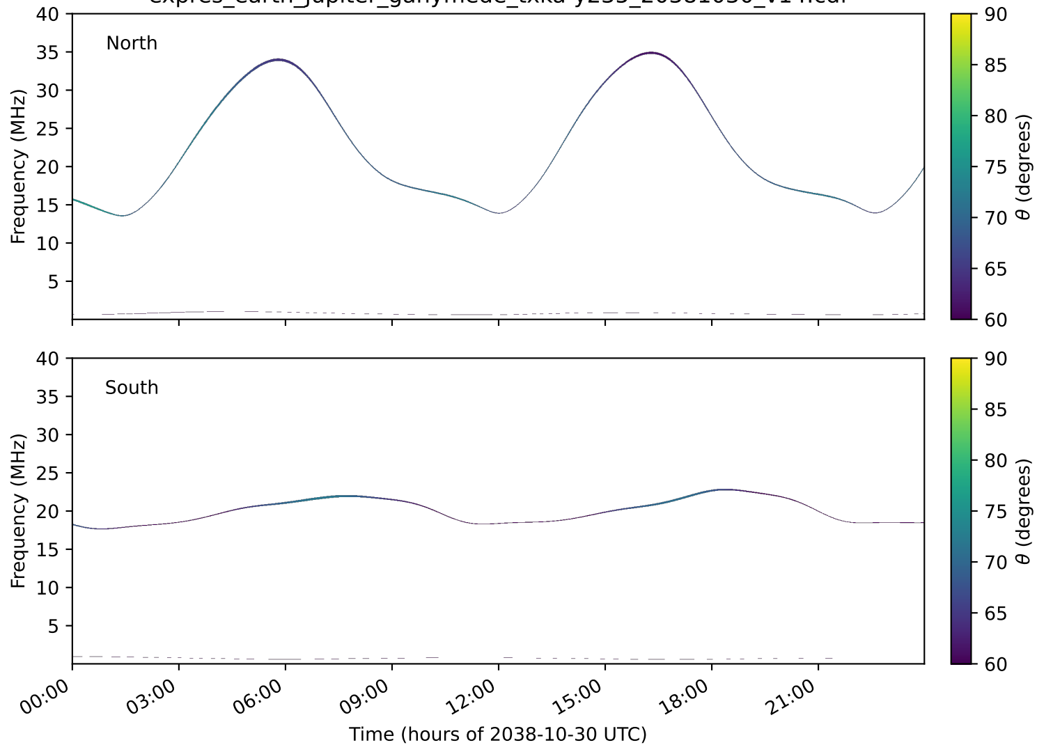
expres_earth_jupiter_ganymede_txka-y235_20381030_v14.cdf
