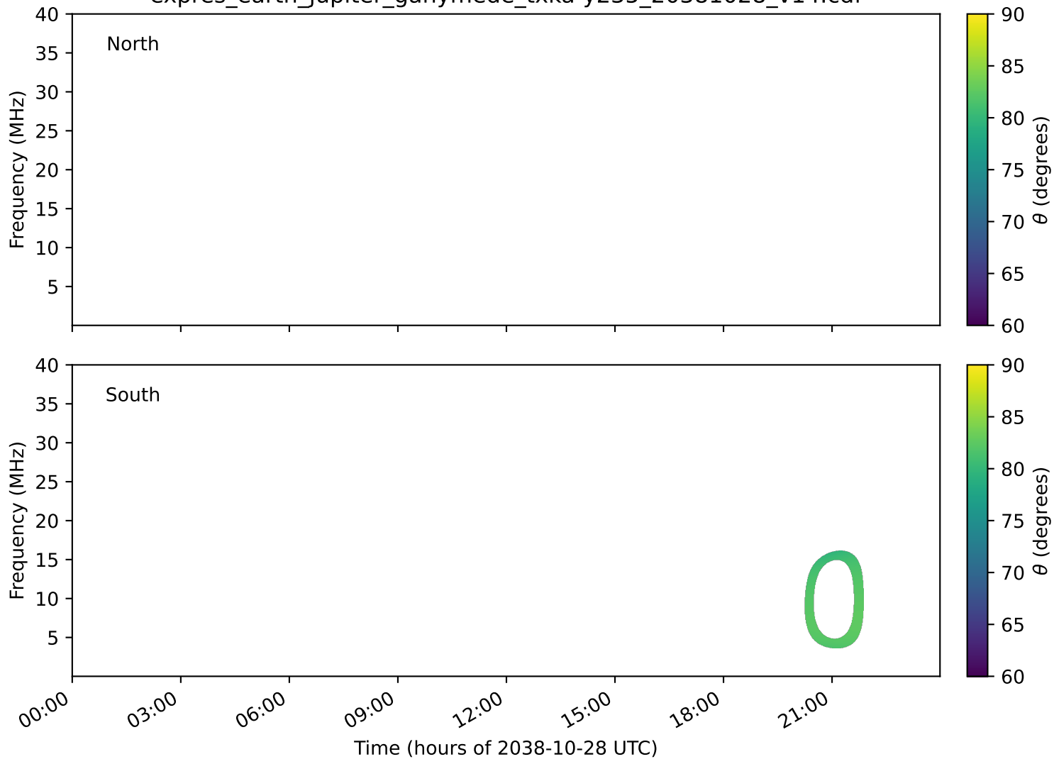
expres_earth_jupiter_ganymede_txka-y235_20381028_v14.cdf
