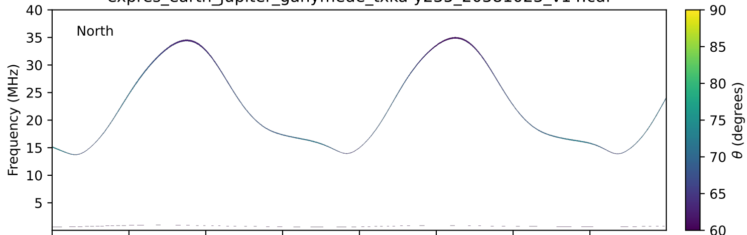
expres_earth_jupiter_ganymede_txka-y235_20381023_v14.cdf
