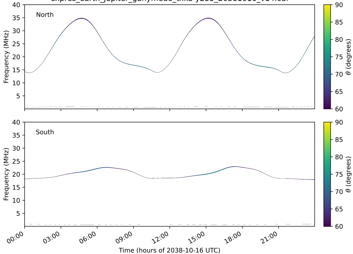
expres_earth_jupiter_ganymede_txka-y235_20381016_v14.cdf
