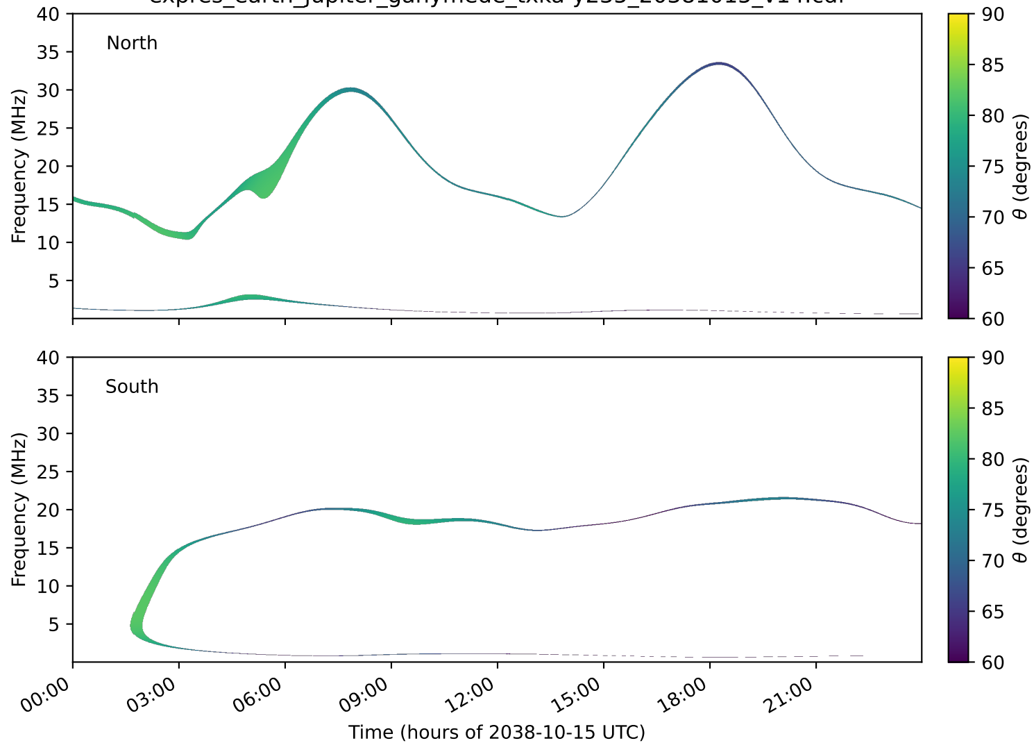
expres_earth_jupiter_ganymede_txka-y235_20381015_v14.cdf
