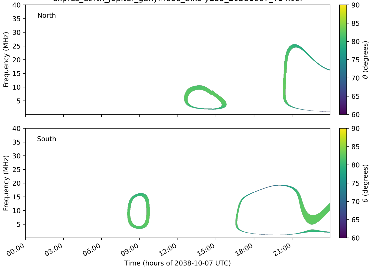
expres_earth_jupiter_ganymede_txka-y235_20381007_v14.cdf
