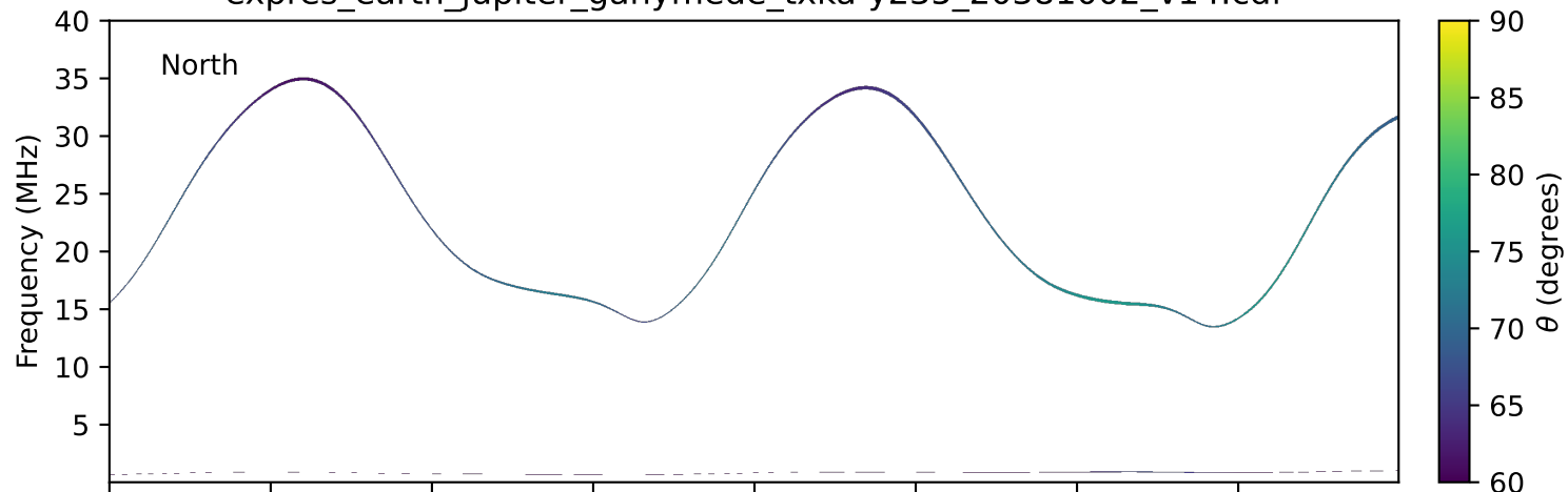
expres_earth_jupiter_ganymede_txka-y235_20381002_v14.cdf
