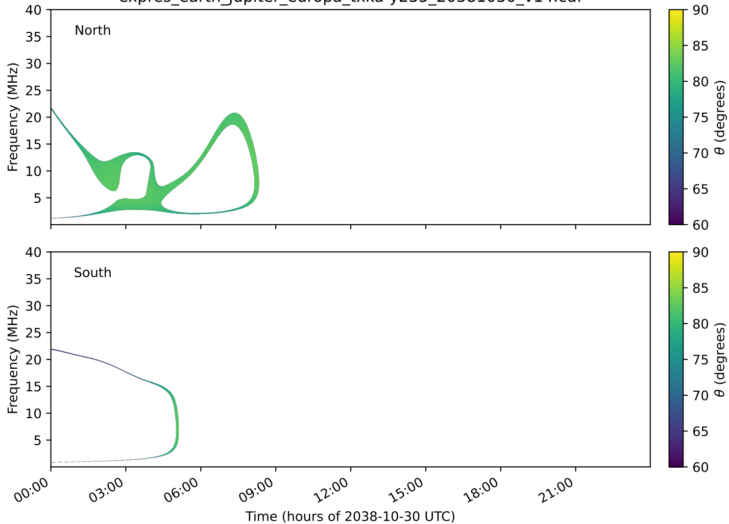
expres_earth_jupiter_europa_txka-y235_20381030_v14.cdf
