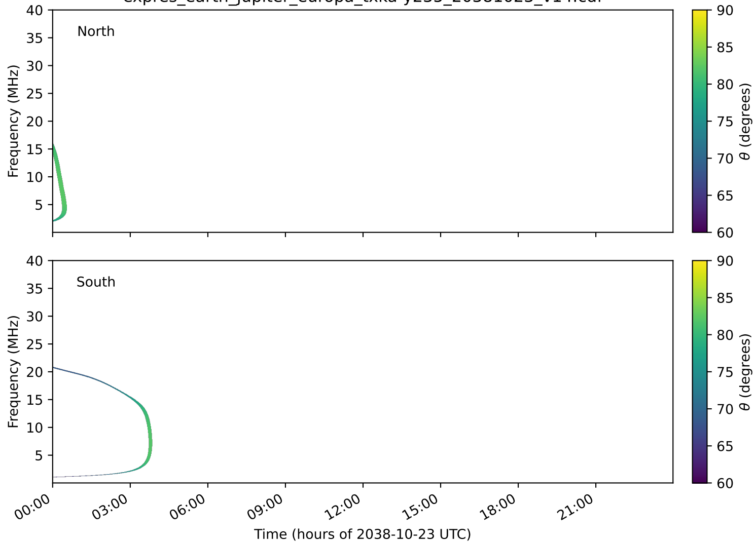
expres_earth_jupiter_europa_txka-y235_20381023_v14.cdf
