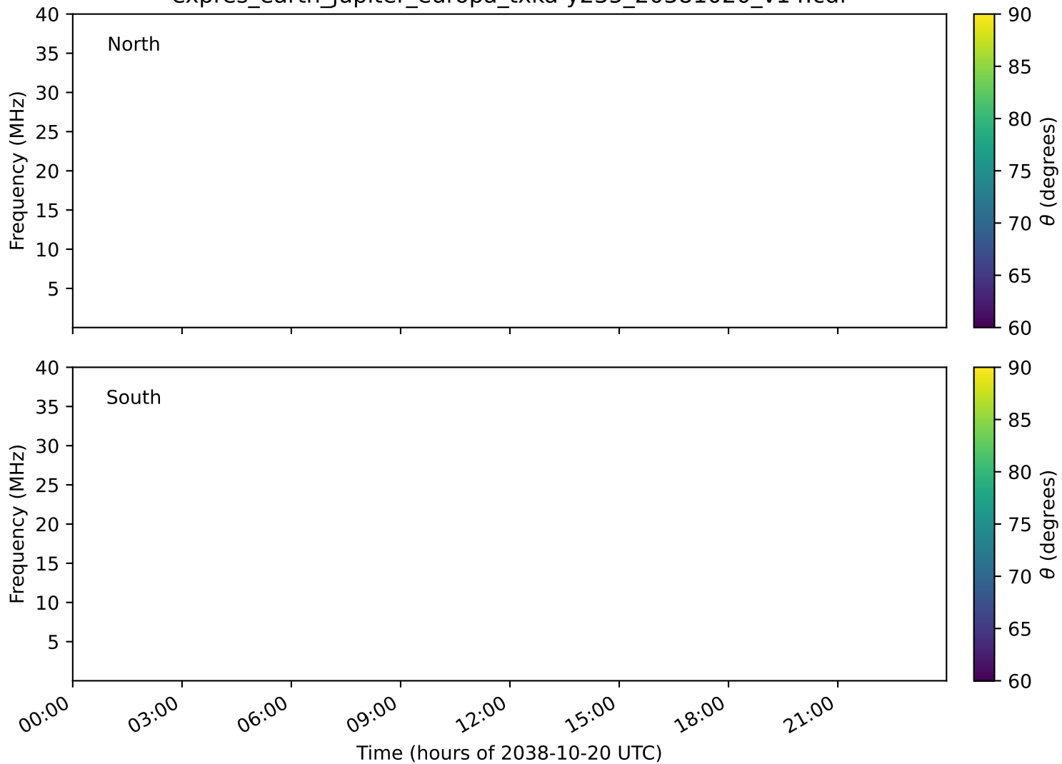
expres_earth_jupiter_europa_txka-y235_20381020_v14.cdf
