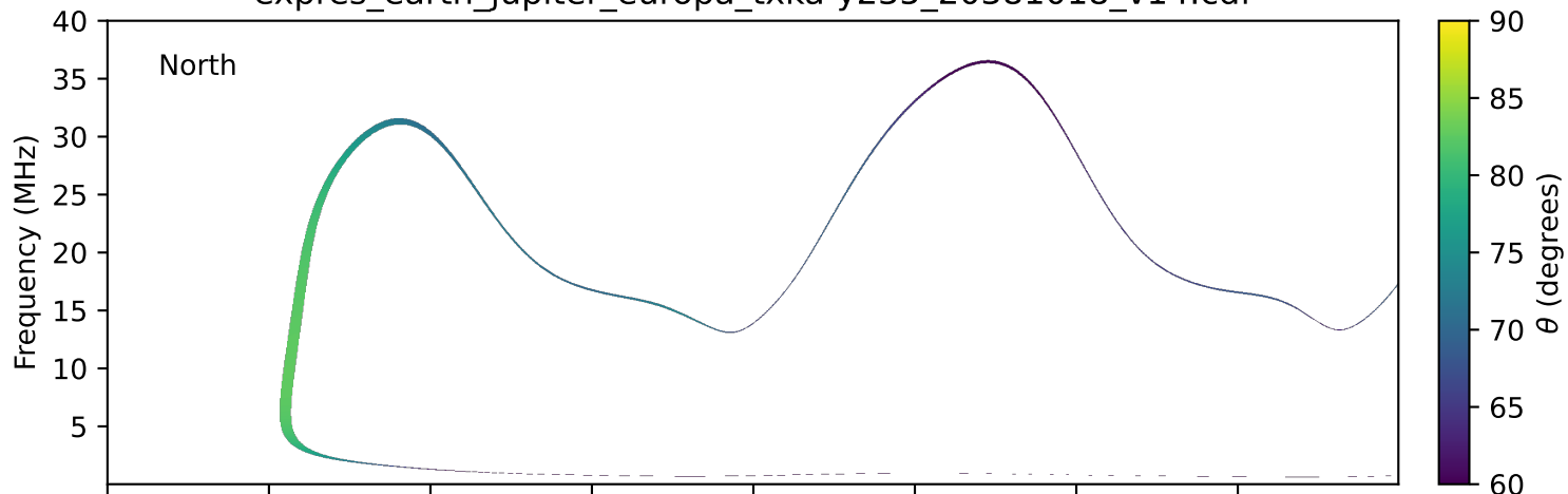
expres_earth_jupiter_europa_txka-y235_20381018_v14.cdf
