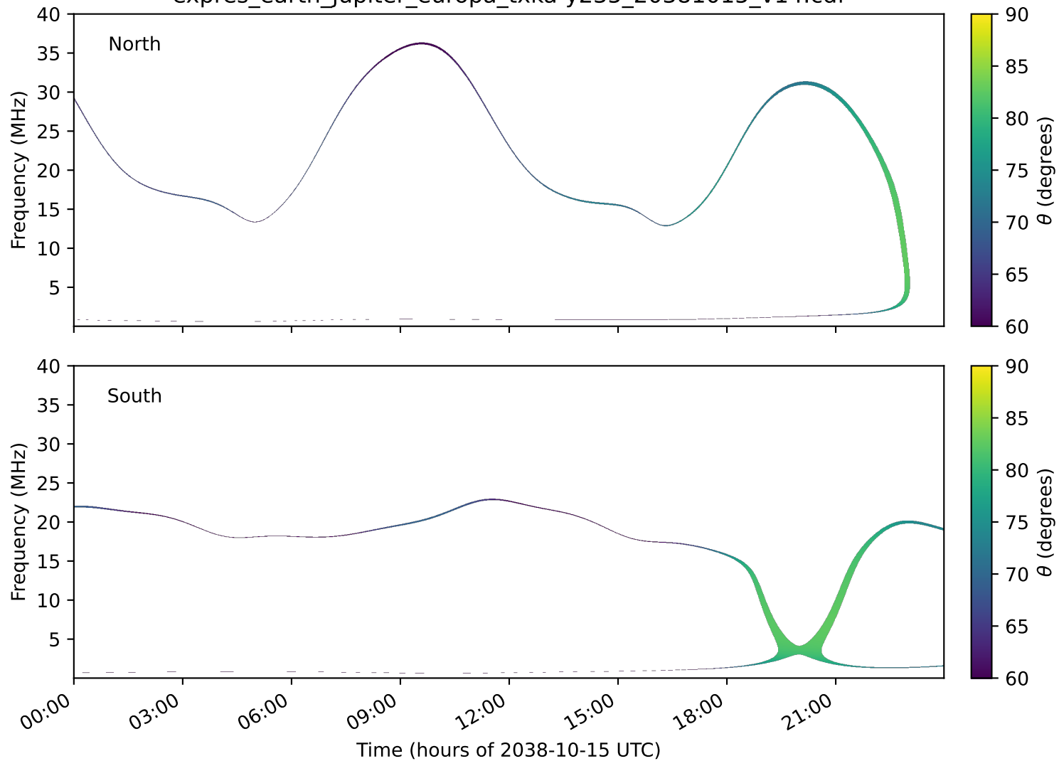
expres_earth_jupiter_europa_txka-y235_20381015_v14.cdf
