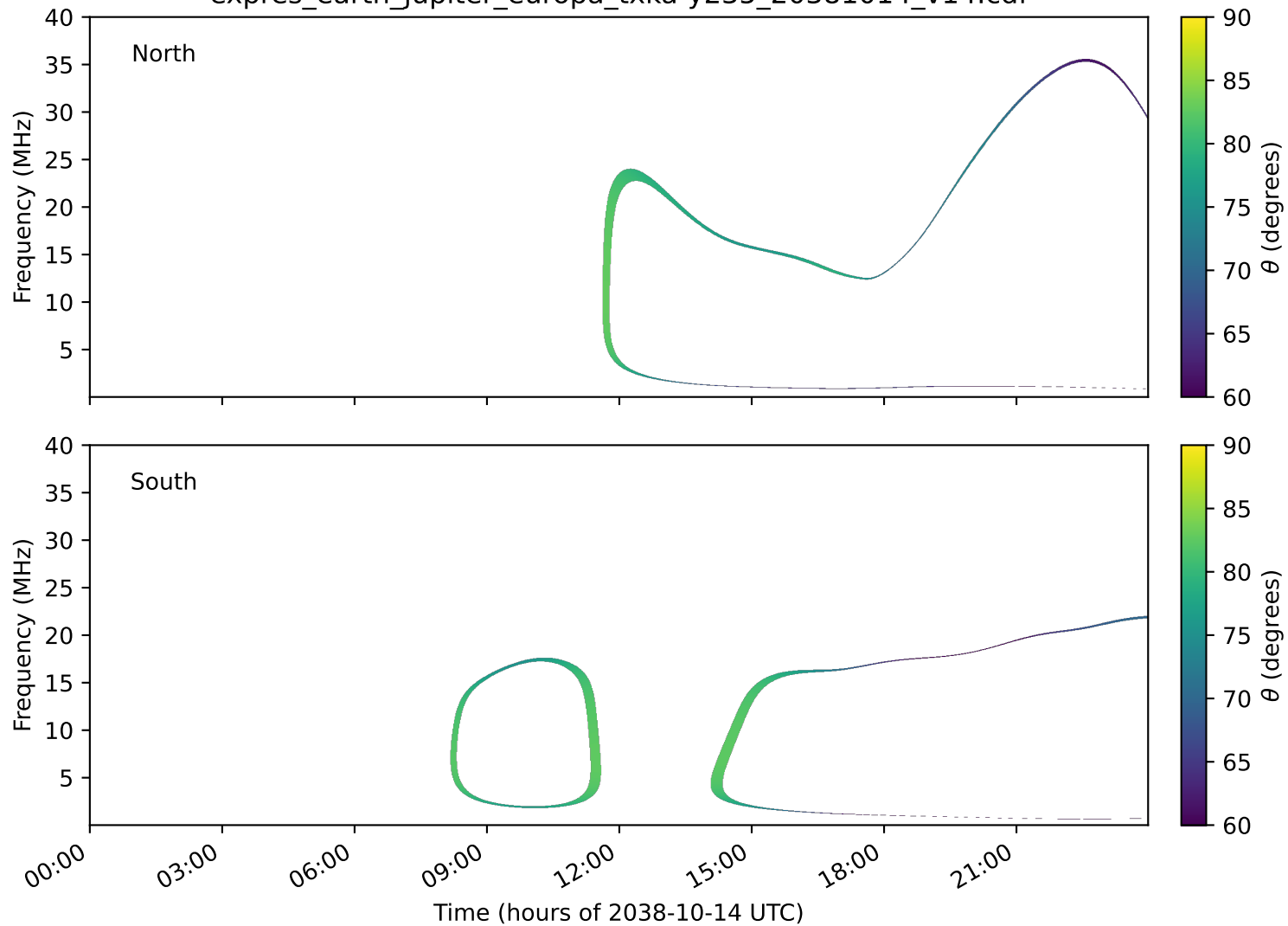
expres_earth_jupiter_europa_txka-y235_20381014_v14.cdf
