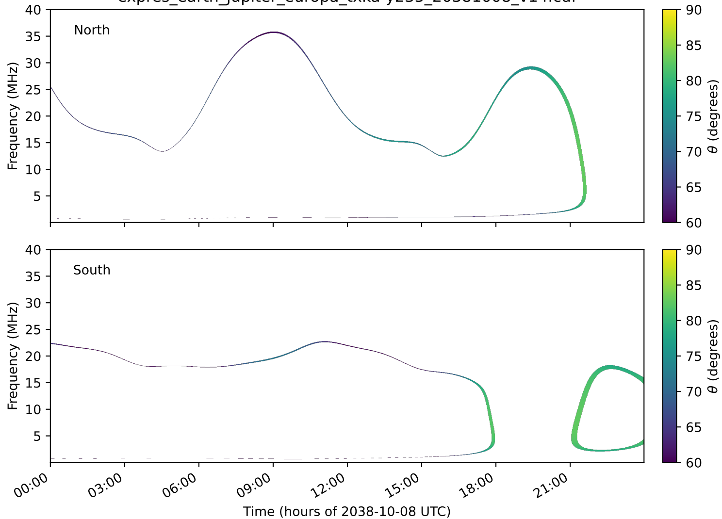
expres_earth_jupiter_europa_txka-y235_20381008_v14.cdf
