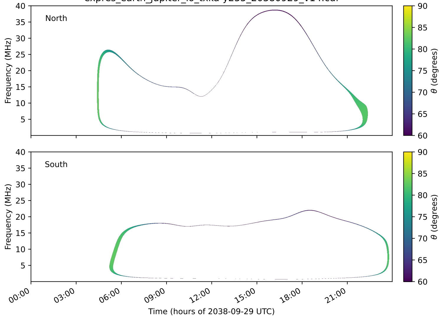
expres_earth_jupiter_io_txka-y235_20380929_v14.cdf
