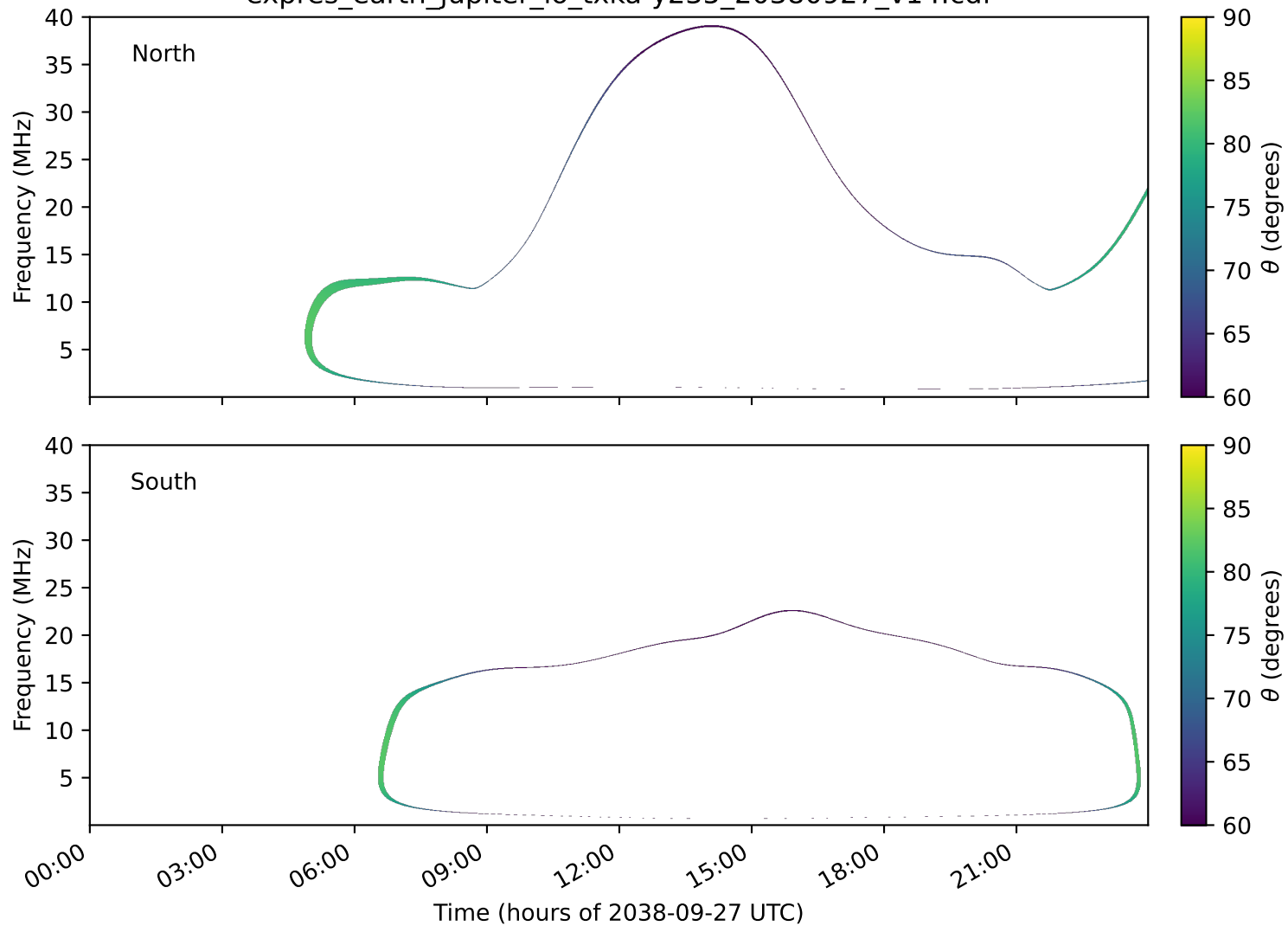
expres_earth_jupiter_io_txka-y235_20380927_v14.cdf
