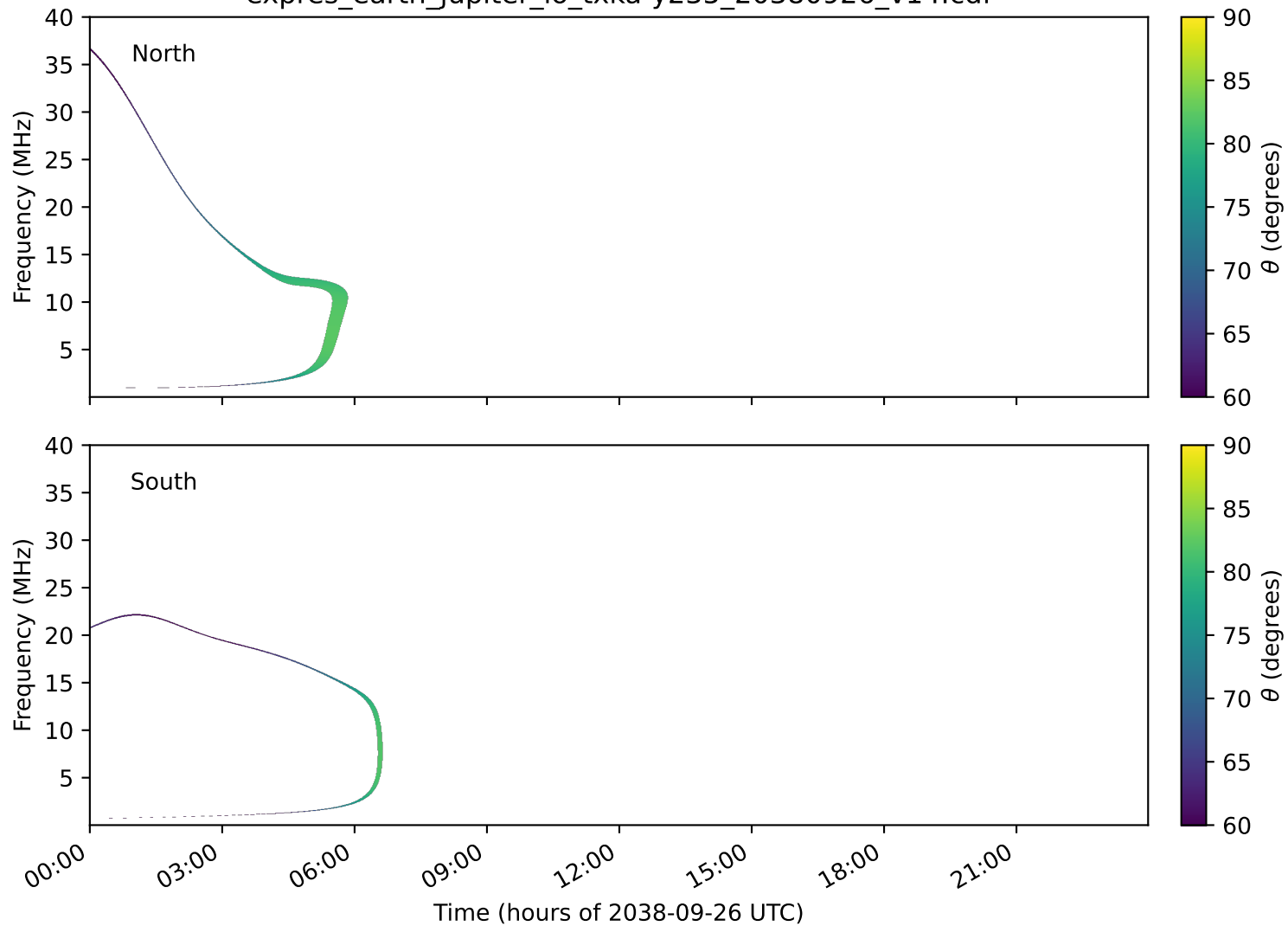
expres_earth_jupiter_io_txka-y235_20380926_v14.cdf
