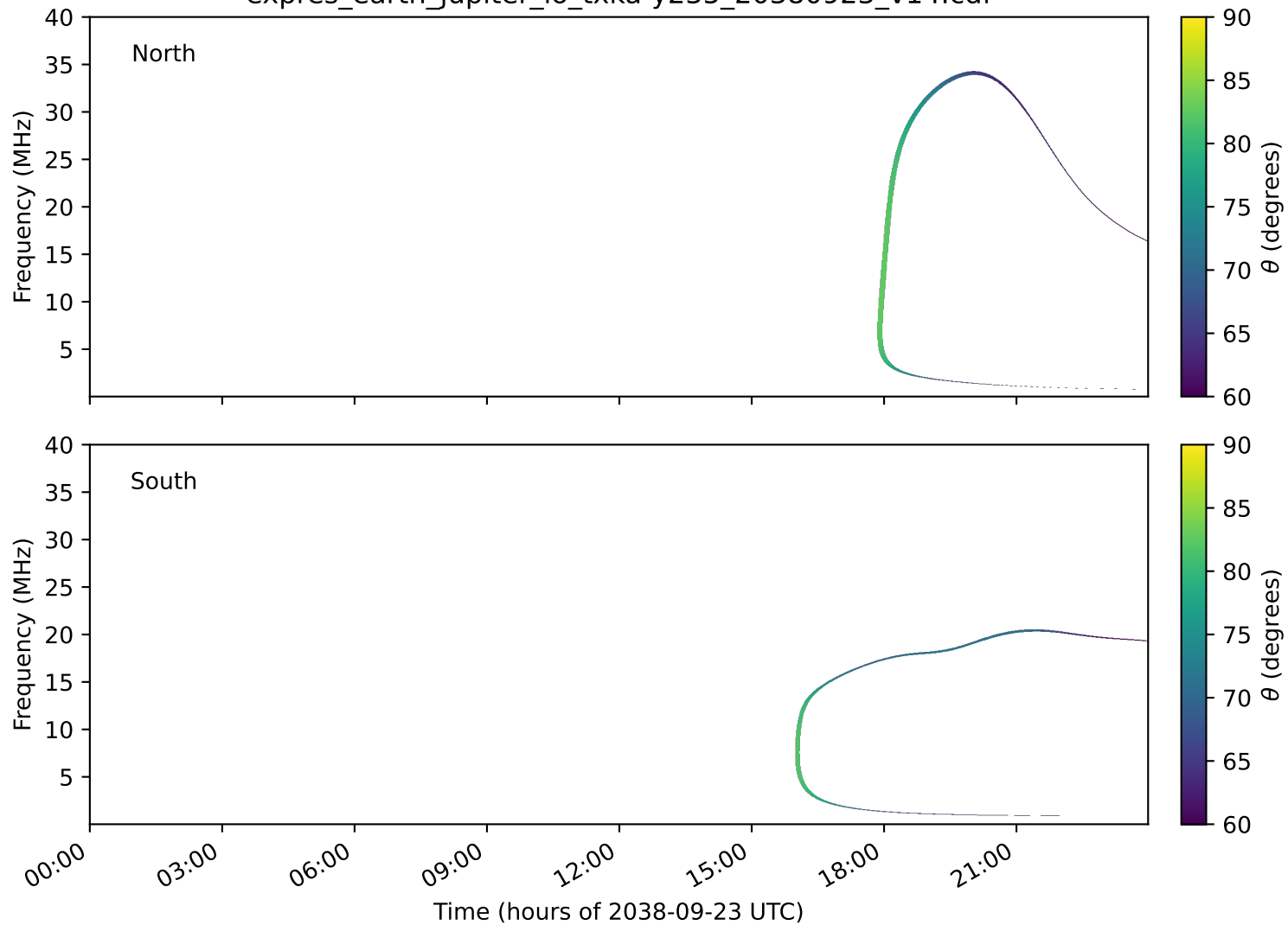
expres_earth_jupiter_io_txka-y235_20380923_v14.cdf
