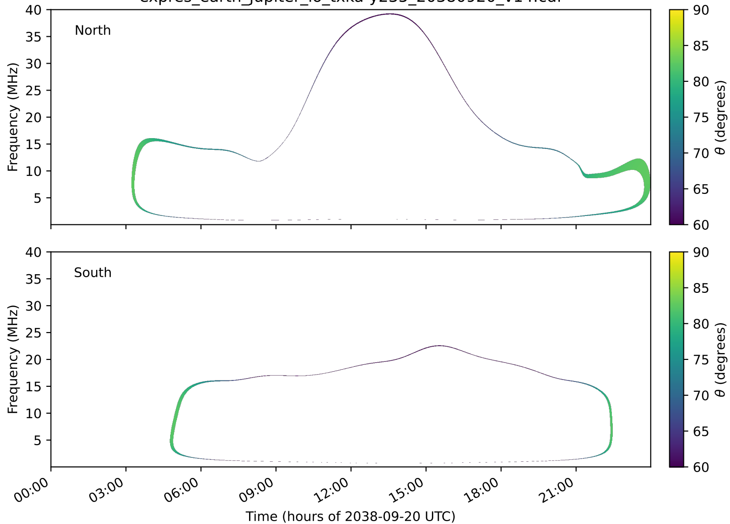
expres_earth_jupiter_io_txka-y235_20380920_v14.cdf
