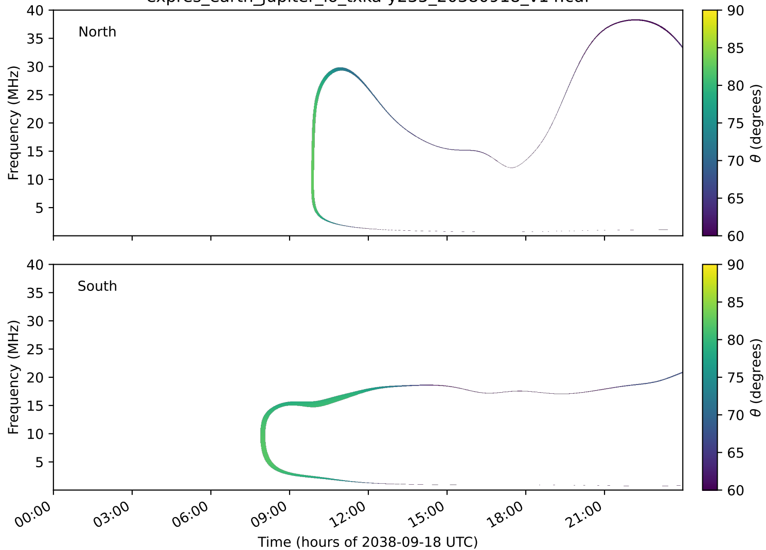
expres_earth_jupiter_io_txka-y235_20380918_v14.cdf
