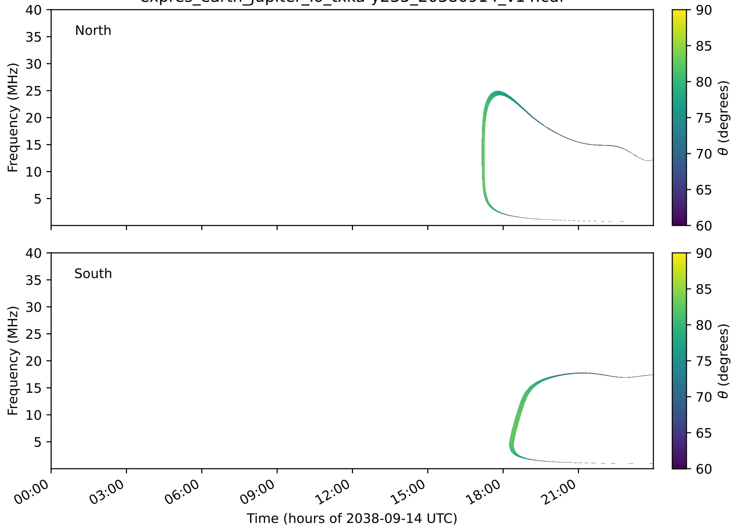
expres_earth_jupiter_io_txka-y235_20380914_v14.cdf
