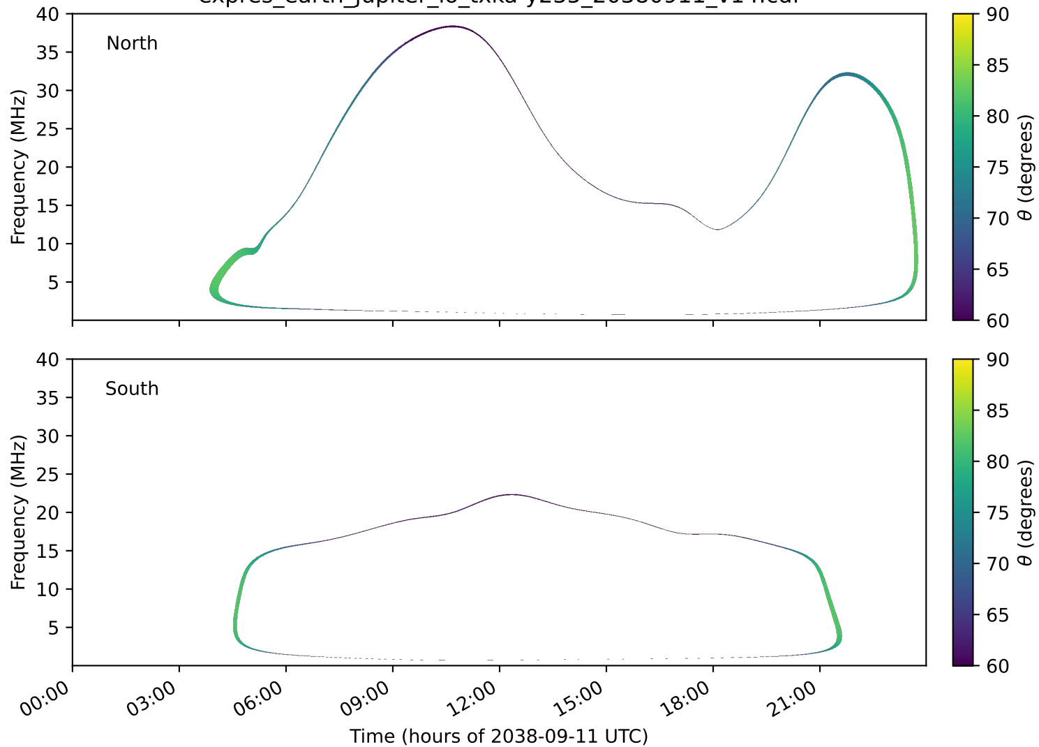
expres_earth_jupiter_io_txka-y235_20380911_v14.cdf
