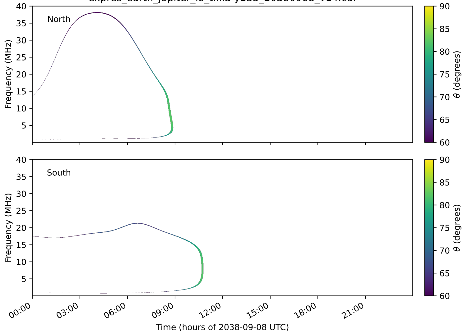
expres_earth_jupiter_io_txka-y235_20380908_v14.cdf
