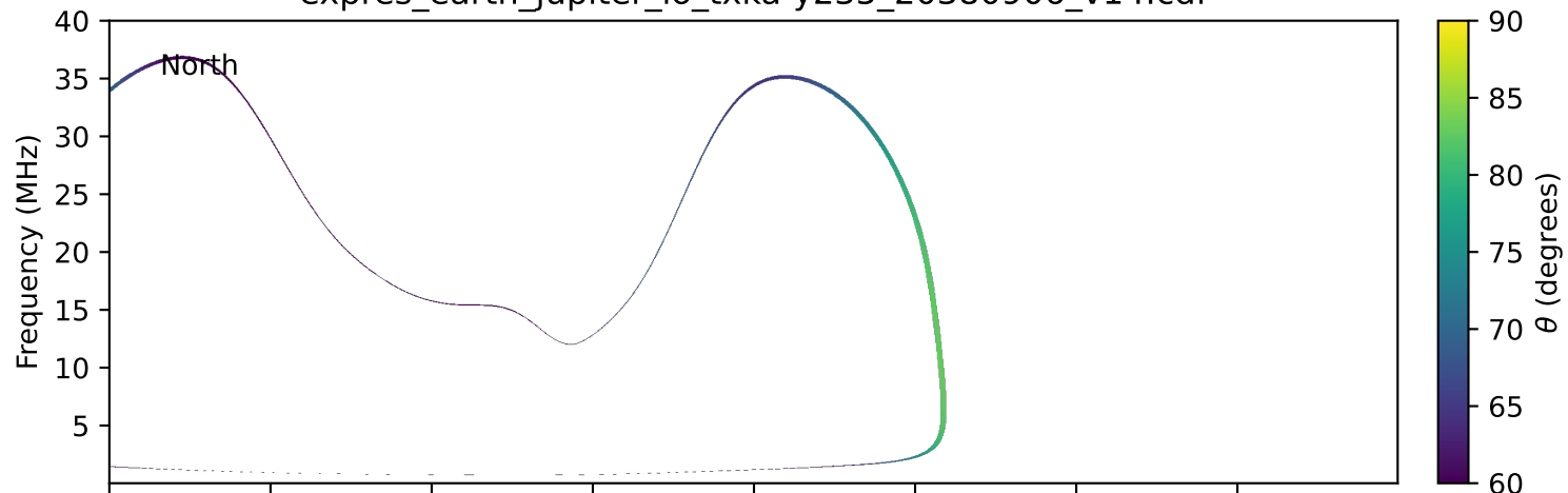
expres_earth_jupiter_io_txka-y235_20380906_v14.cdf
