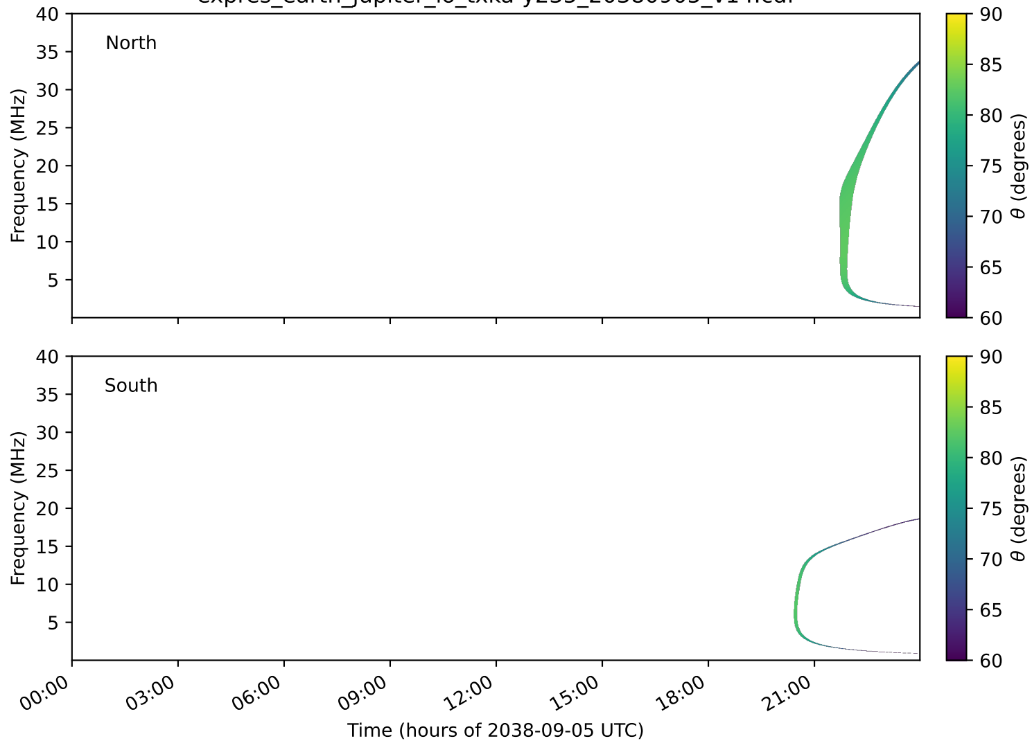
expres_earth_jupiter_io_txka-y235_20380905_v14.cdf
