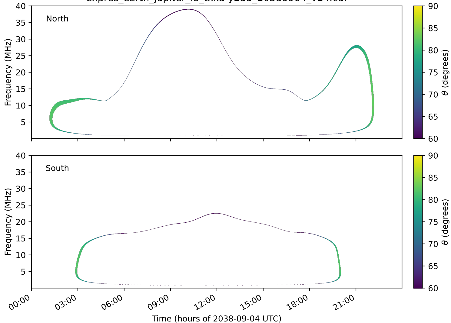
expres_earth_jupiter_io_txka-y235_20380904_v14.cdf
