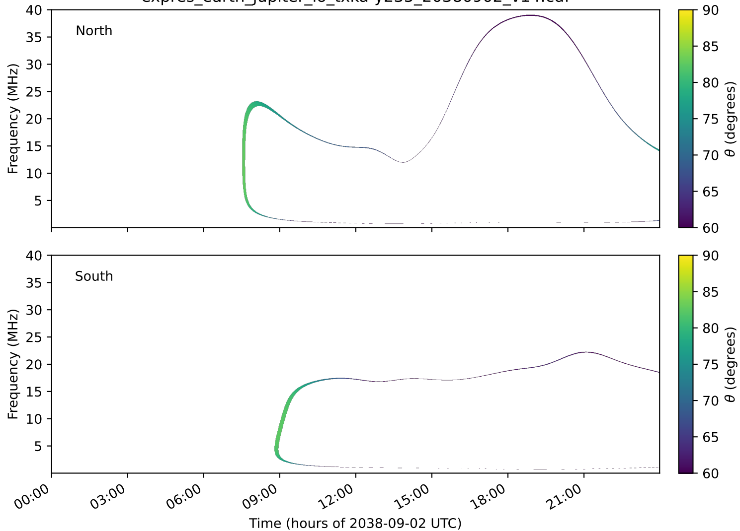
expres_earth_jupiter_io_txka-y235_20380902_v14.cdf
