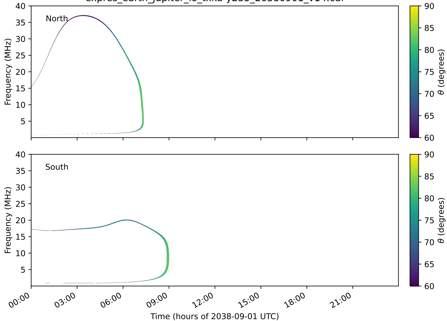
expres_earth_jupiter_io_txka-y235_20380901_v14.cdf
