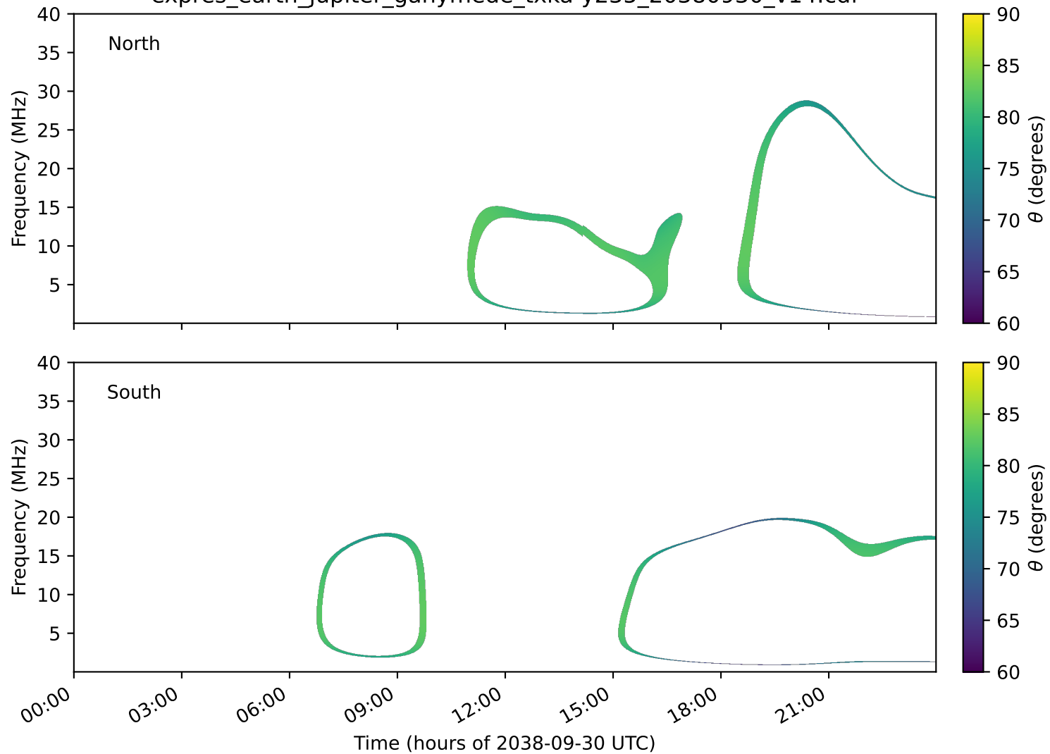
expres_earth_jupiter_ganymede_txka-y235_20380930_v14.cdf
