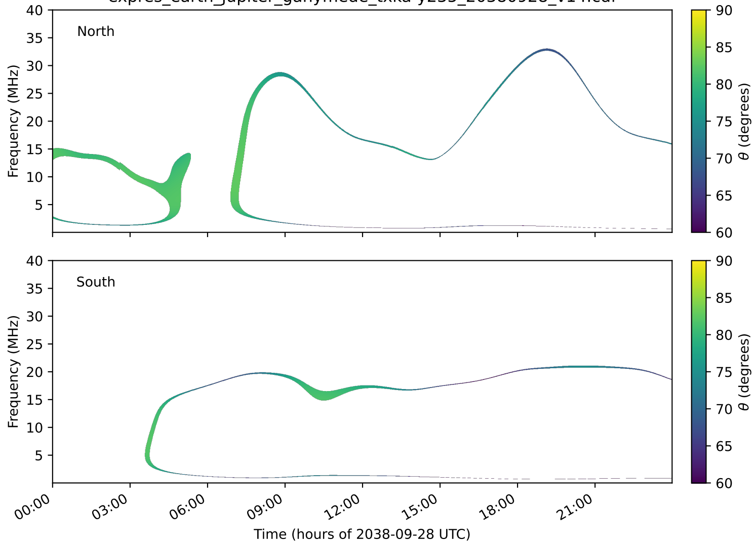
expres_earth_jupiter_ganymede_txka-y235_20380928_v14.cdf
