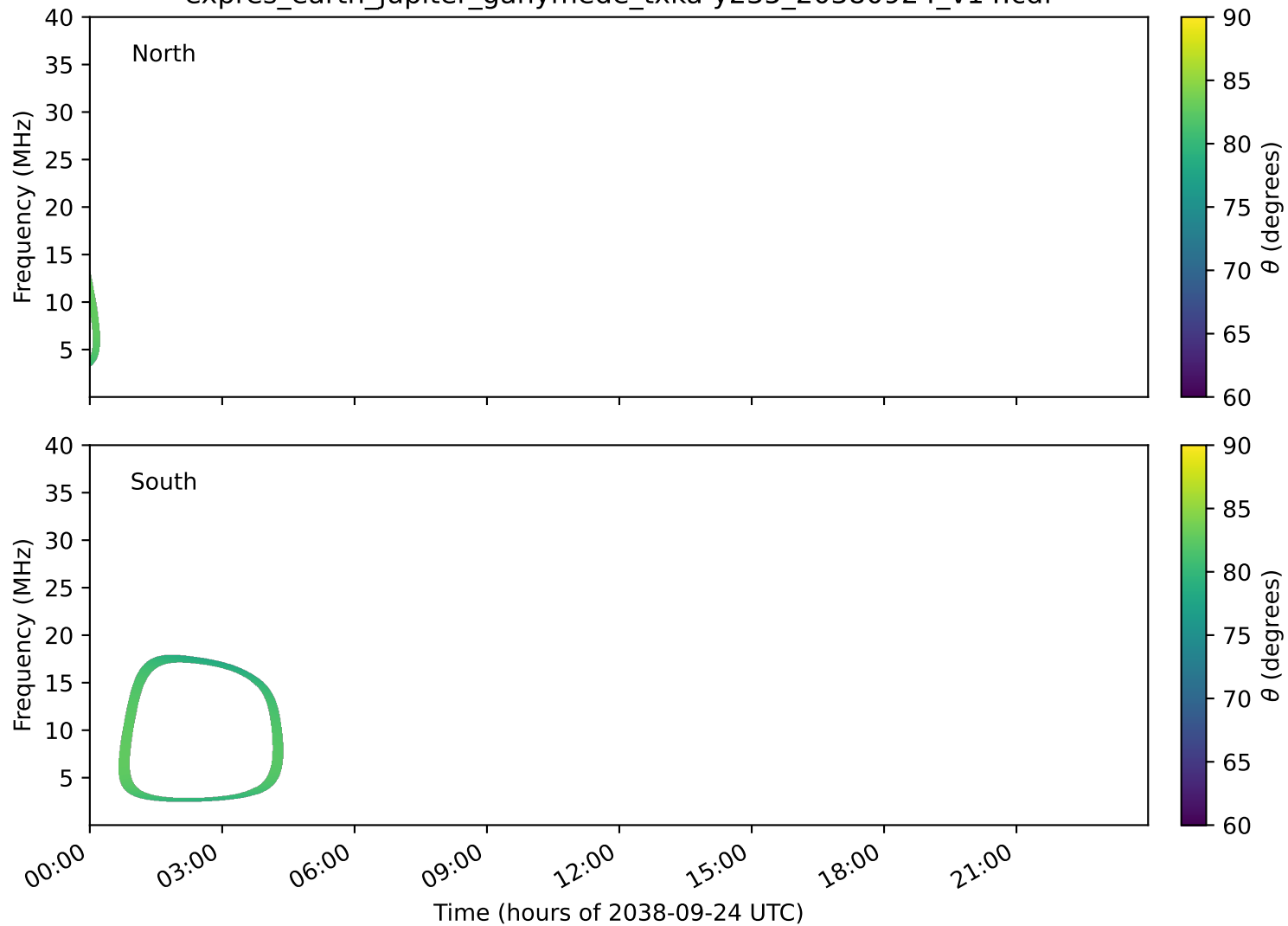
expres_earth_jupiter_ganymede_txka-y235_20380924_v14.cdf
