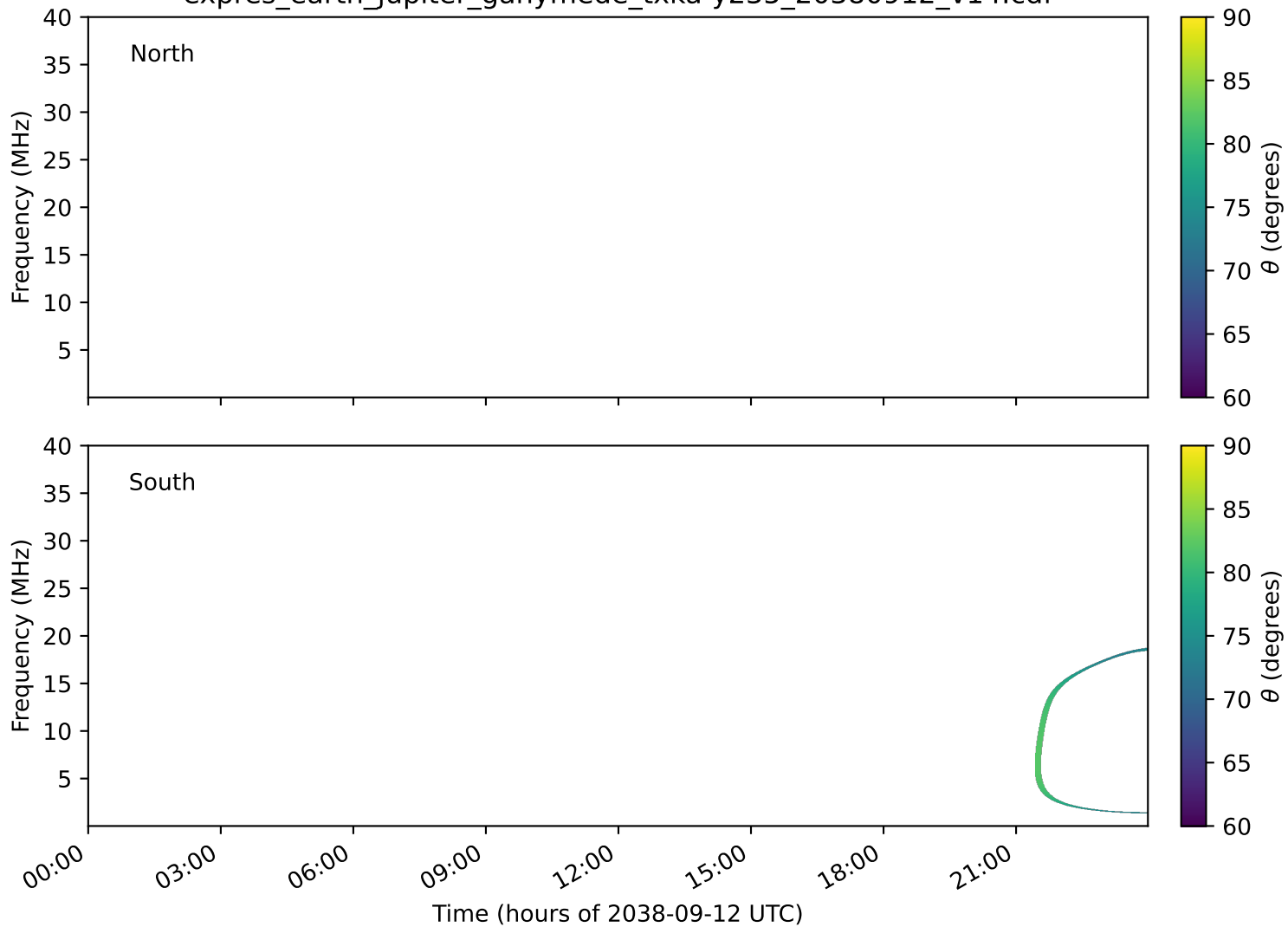
expres_earth_jupiter_ganymede_txka-y235_20380912_v14.cdf
