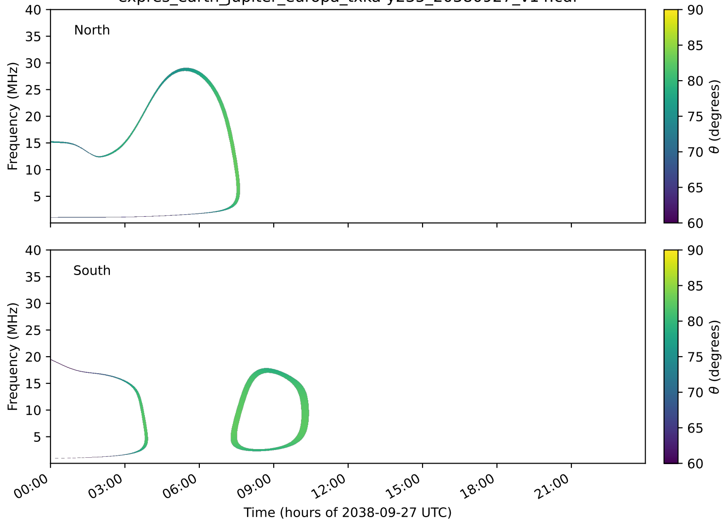
expres_earth_jupiter_europa_txka-y235_20380927_v14.cdf
