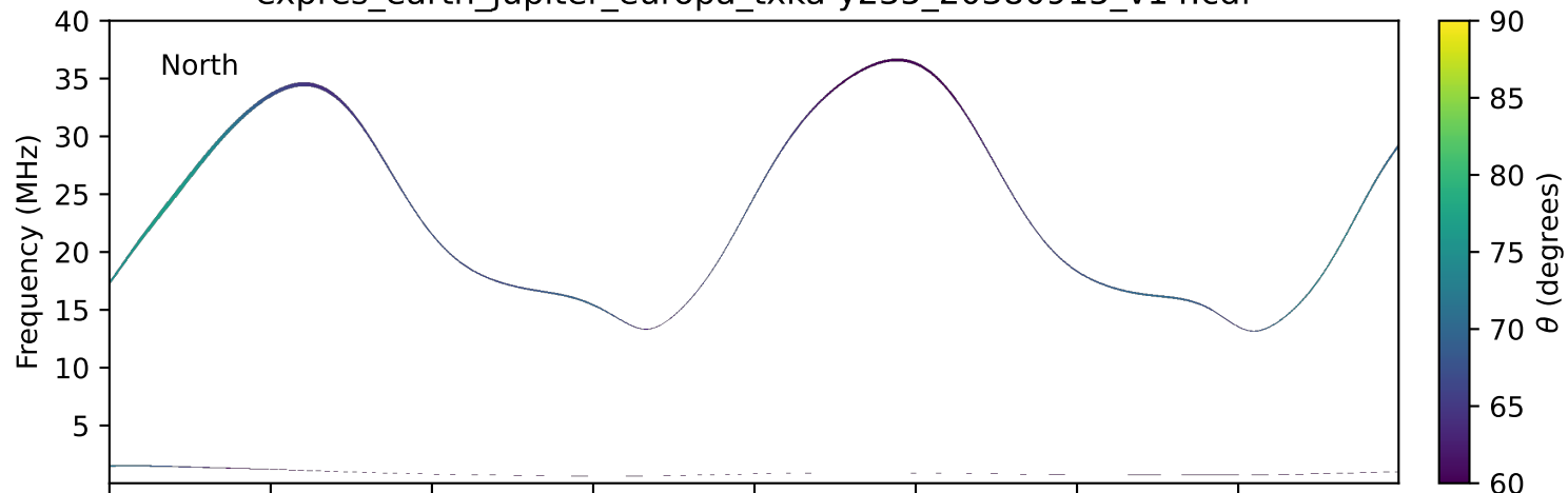
expres_earth_jupiter_europa_txka-y235_20380915_v14.cdf
