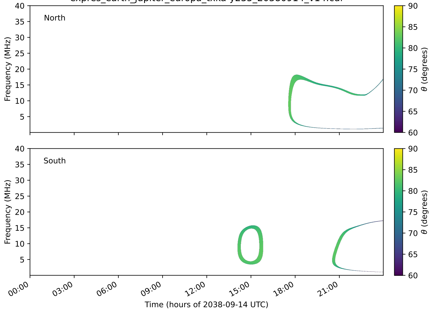
expres_earth_jupiter_europa_txka-y235_20380914_v14.cdf
