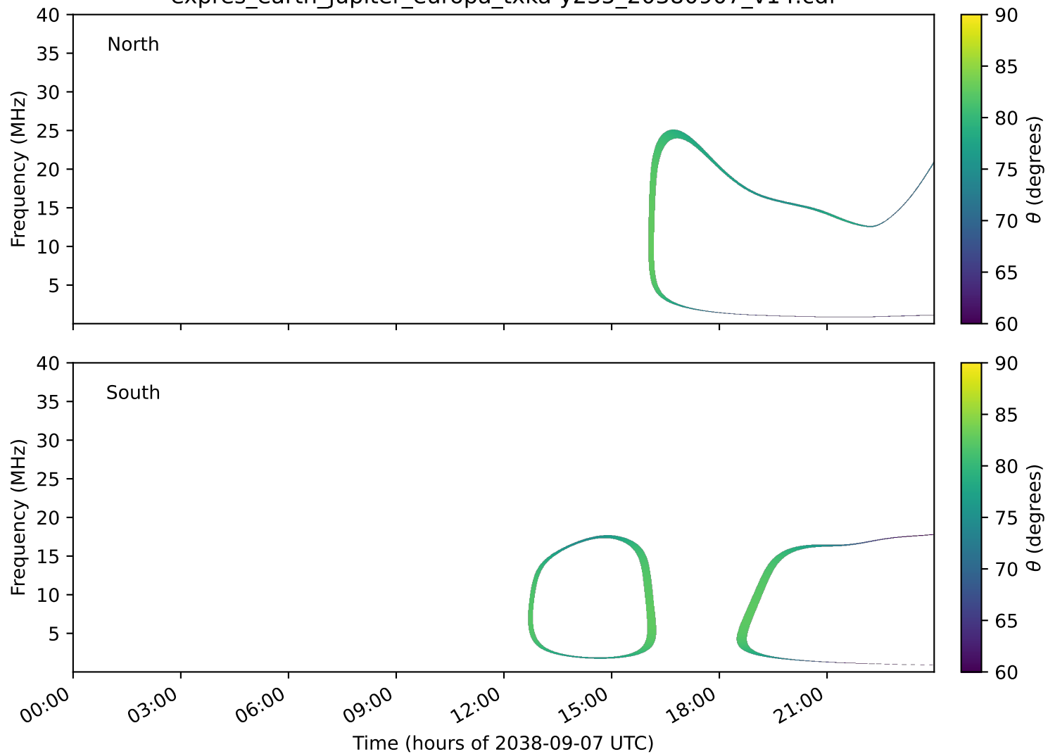
expres_earth_jupiter_europa_txka-y235_20380907_v14.cdf
