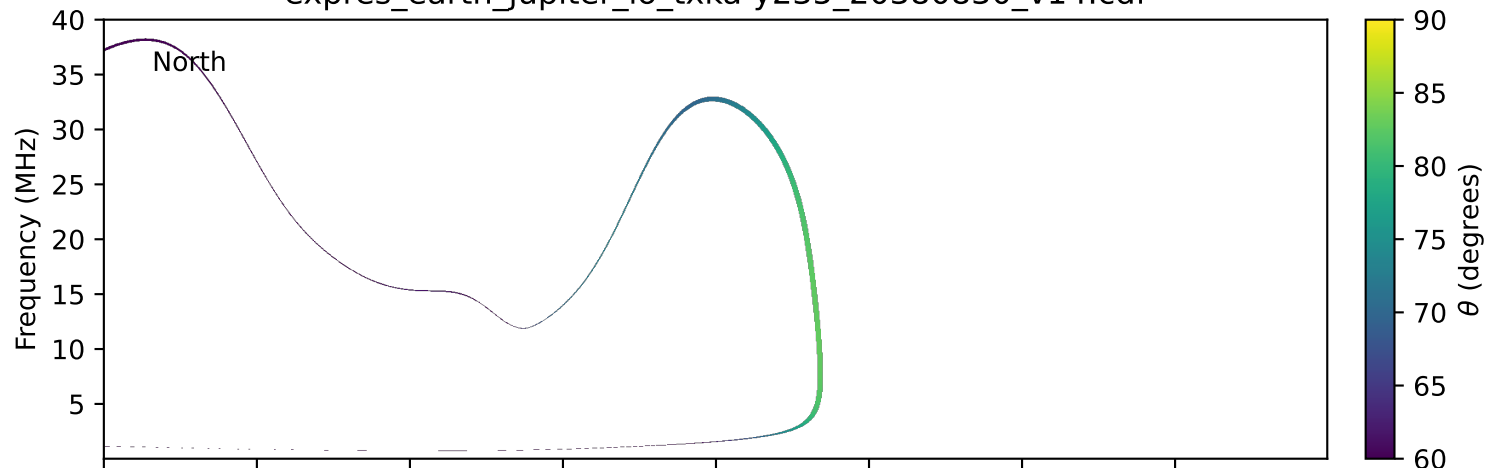
expres_earth_jupiter_io_txka-y235_20380830_v14.cdf
