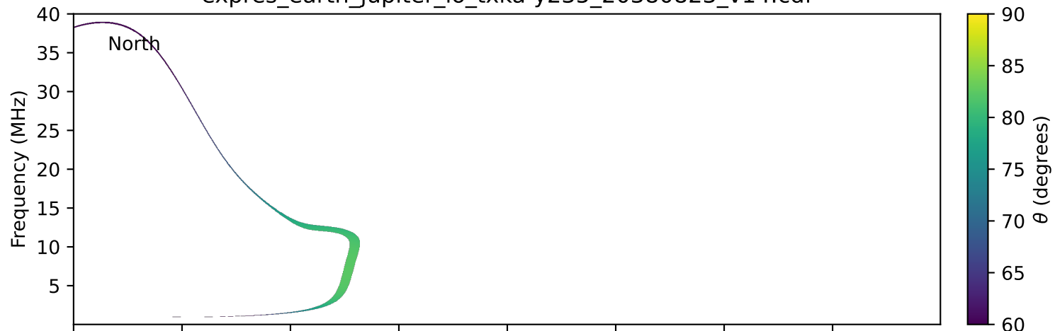
expres_earth_jupiter_io_txka-y235_20380823_v14.cdf
