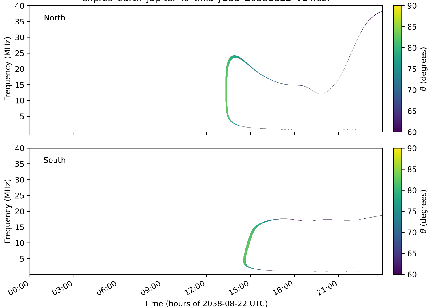
expres_earth_jupiter_io_txka-y235_20380822_v14.cdf
