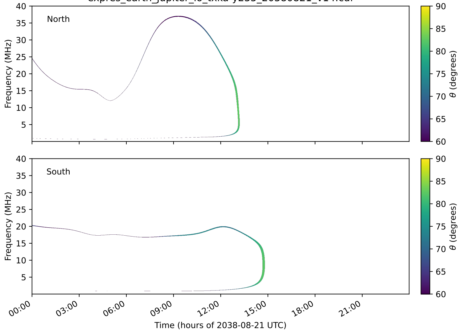
expres_earth_jupiter_io_txka-y235_20380821_v14.cdf
