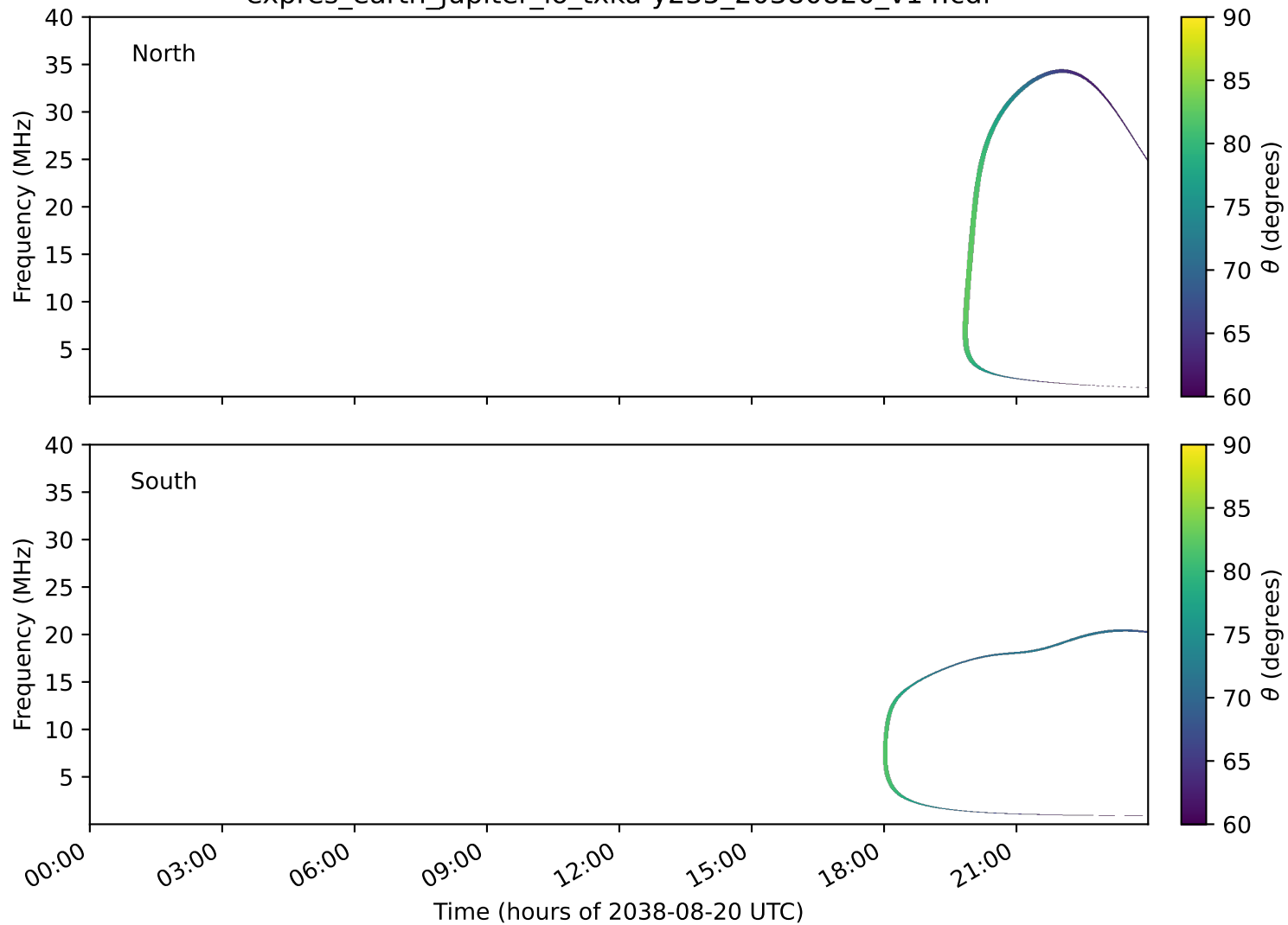
expres_earth_jupiter_io_txka-y235_20380820_v14.cdf
