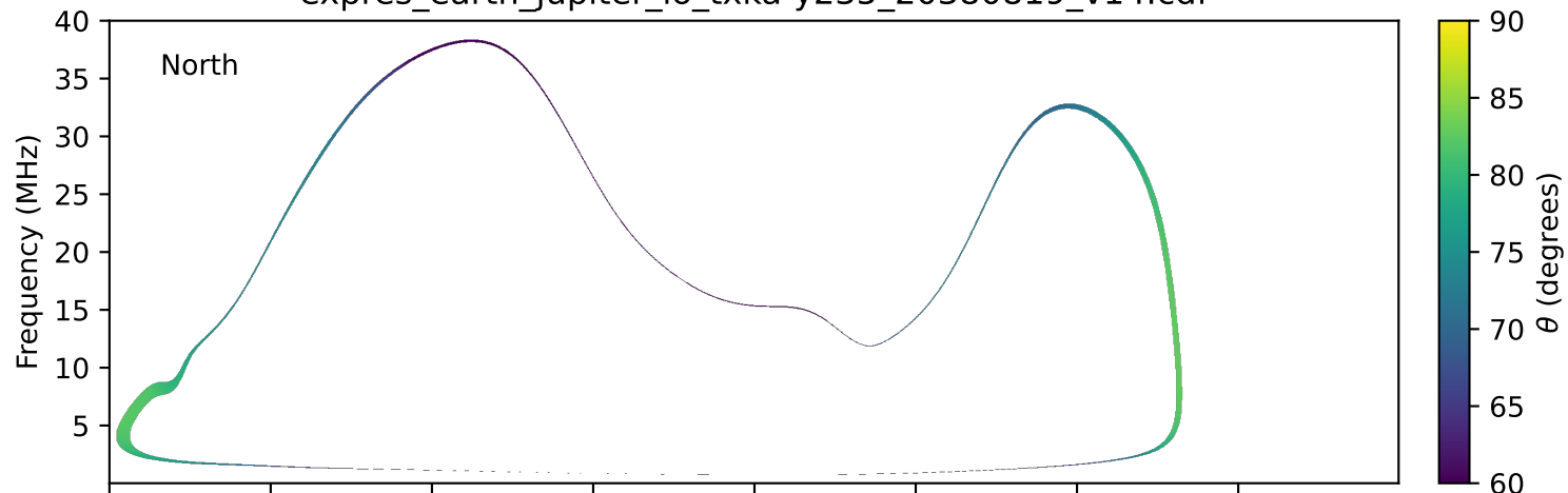
expres_earth_jupiter_io_txka-y235_20380819_v14.cdf
