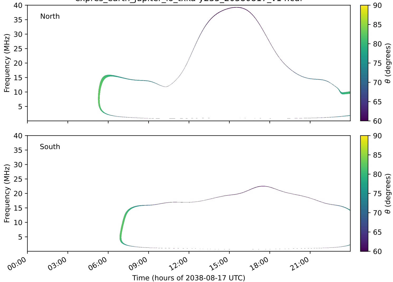
expres_earth_jupiter_io_txka-y235_20380817_v14.cdf
