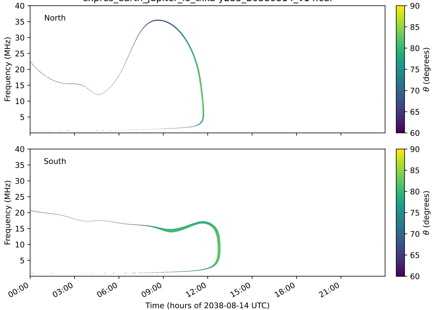
expres_earth_jupiter_io_txka-y235_20380814_v14.cdf
