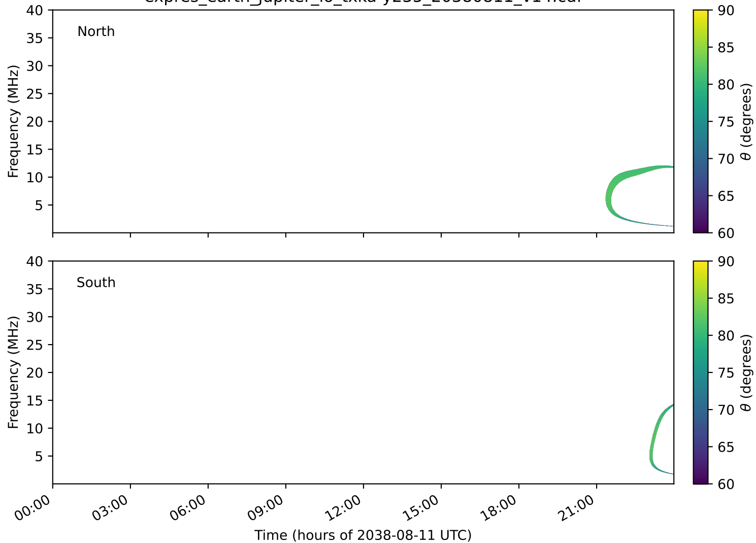
expres_earth_jupiter_io_txka-y235_20380811_v14.cdf
