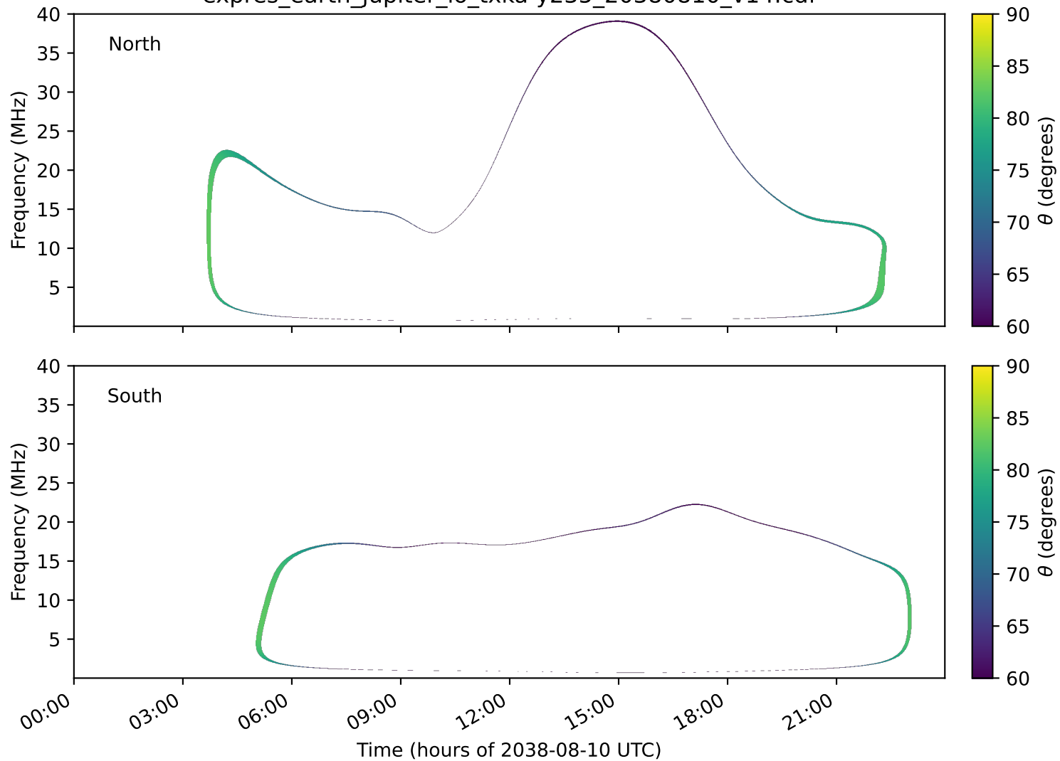
expres_earth_jupiter_io_txka-y235_20380810_v14.cdf
